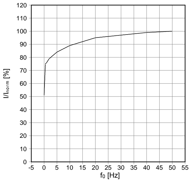
fo - derating curves IGBT (motor) \cos(\phi) = 0,85 , (motor) T_{cool\ medium} = 40^{\circ}C
